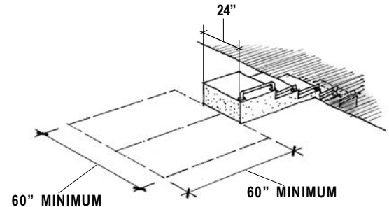
CLEAR DECK SPACE LOCATED AT A TRANSFER SYSTEM
