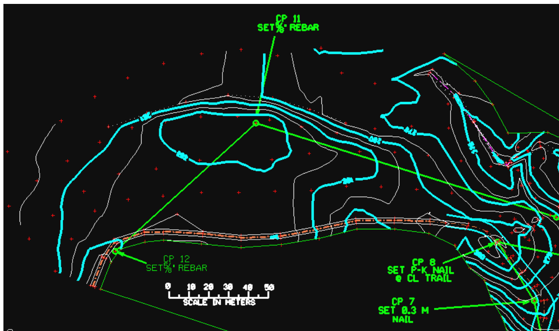
Figure F-5. Western portion of survey area
