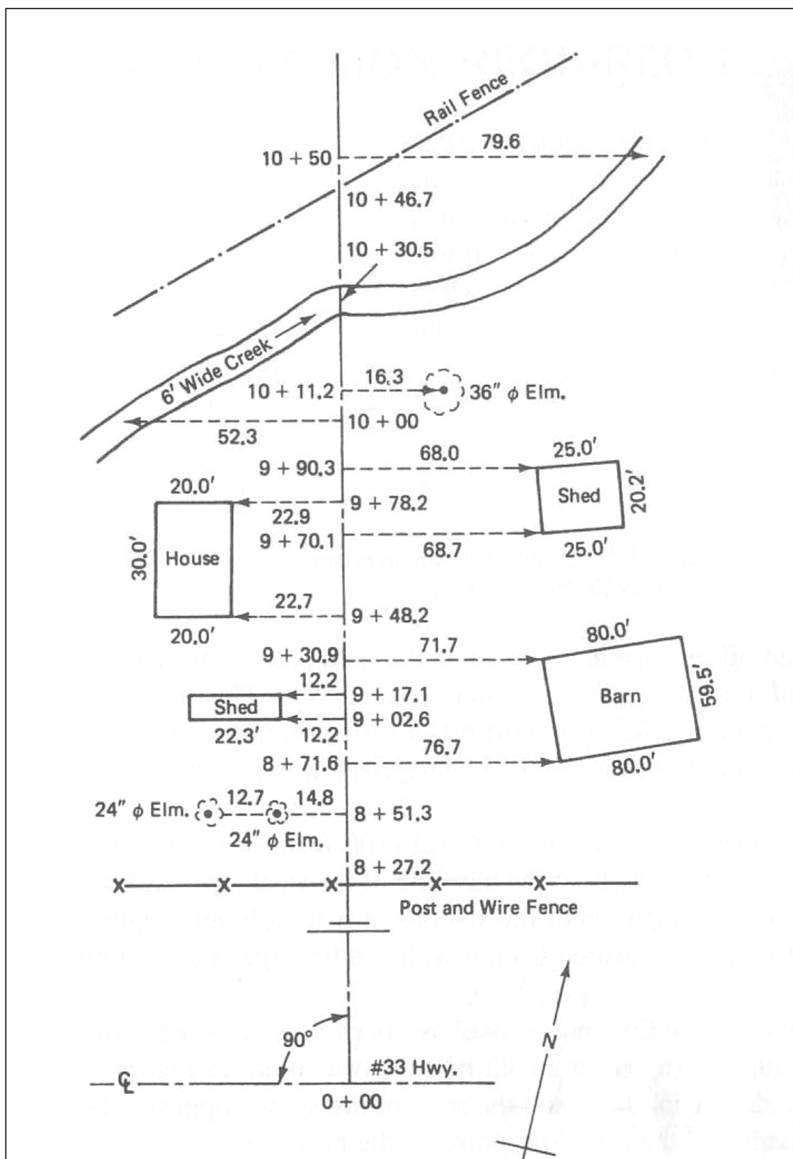
Figure 2-10. Sketch of profile line and cross-section (Kavanagh 1997)
