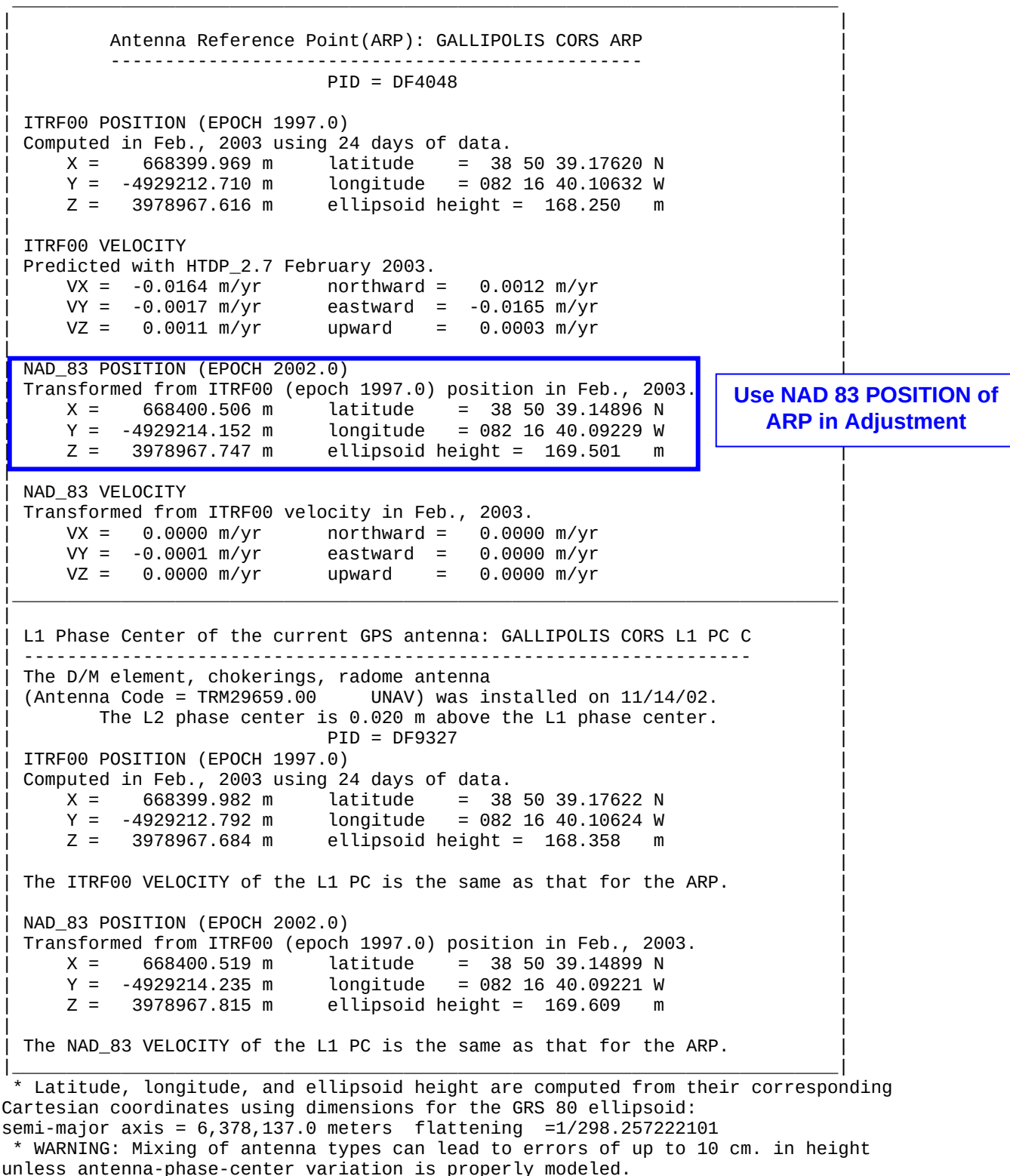
Figure 6-9. CORS antenna reference data
