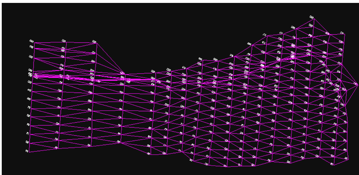
Figure E-1. TIN/DTM of surveyed cross-sections showing 18 cross-sections spaced at 50 ft and 100 ft C/C
