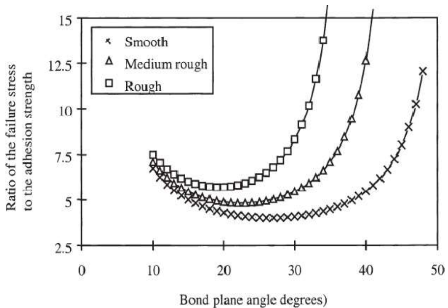
Figure 4.11. Influence of bond plane angle and roughness on failure stress (Austin et al., 1999)
