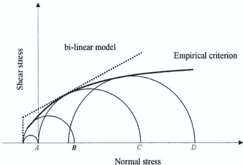
Figure 4.5. Mohr's circle from A: direct tension B: Brazilian test C: unconfined compression, D tri axial compression tests (Austin et al., 1999).
