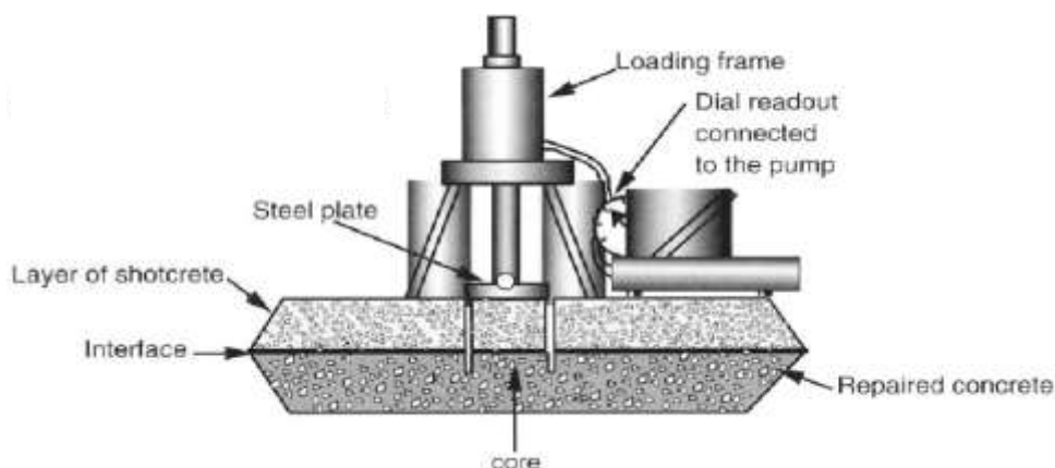
Figure 4.6. Pull-off test procedure (Beaupre, 1999)
