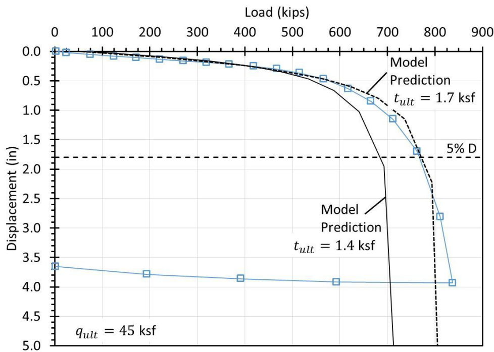
Figure 10.22: Load-settlement response for Test Shaft TS-5.
