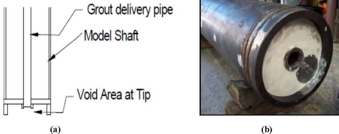
Figure 5.7: Low mobility grouting device: (a) schematic, and (b) photograph of device used for laboratory-scale tests (Pooranampillai, 2010).
