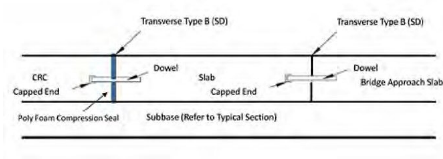
Figure 49. Transition from CRCP using doweled joints.
