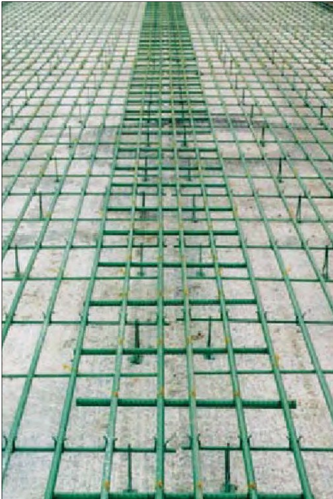
Figure 27. Planned location and tie bars for saw-cut longitudinal joint.
