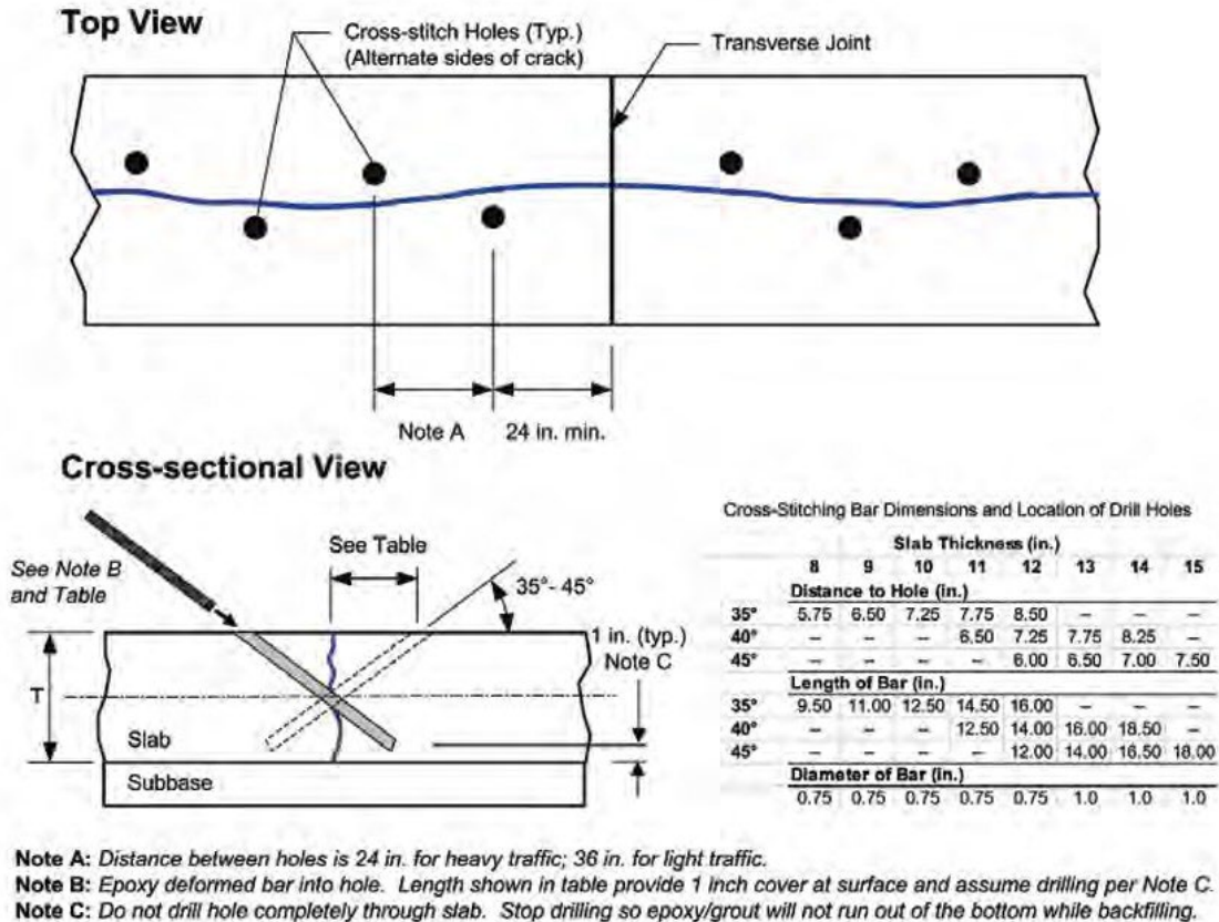
Figure 75. Cross-stitching a longitudinal crack.
