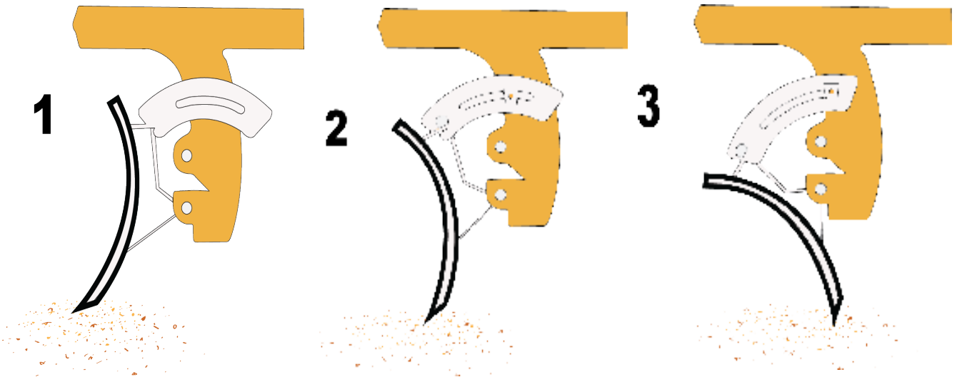
FIGURE 2: Moldboard pitch.
