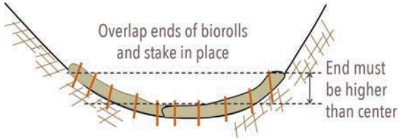
Figure 21: Proper check dam installation
