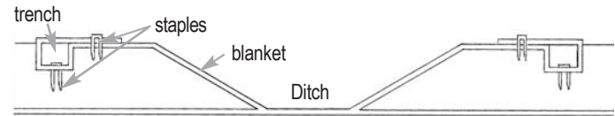
Figure 15: Example staple patterns
