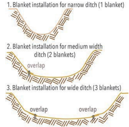
Figure 17: How to install single and multiple ditch blankets. Four to six inch overlap on side seams.
