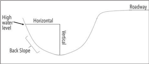
Figure 40: Measuring H:V ratio for back slope
