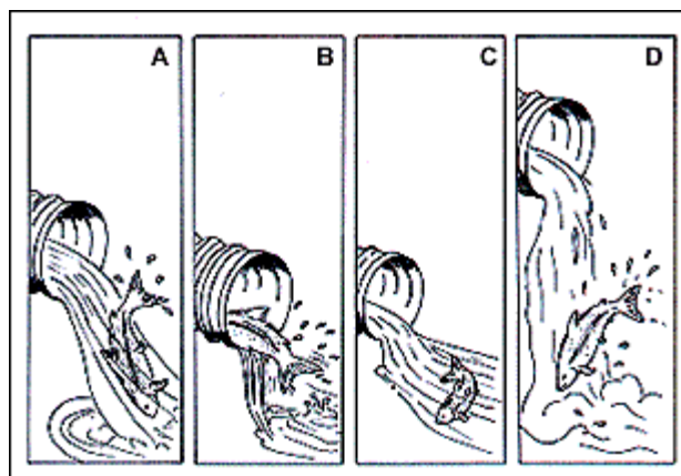
Figure 21. Improperly installed culverts can block fish passage: (A) water velocity too great, (B) water in culvert too shallow, (C) no resting pool below culvert,
