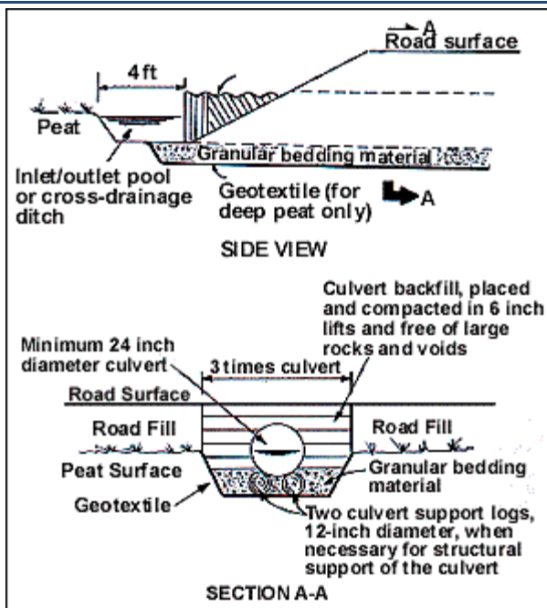
Figure 24. Proper culvert height is lower in wetlands than in other forest conditions, to accommodate subsurface flow. (Redrawn and adapted from Minnesota Department of Natural Resources 1995, p. 55)
