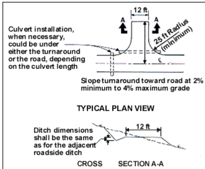
Figure 8. Turnaround design should consider drainage.
