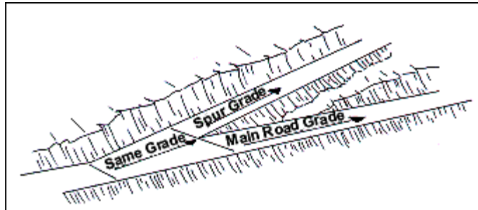
Figure 5. A main road and spur must have the same grade for a distance equal to at least the sum of half the width of each. (Redrawn and adapted from Figure 2.4-7, Darrach et al. 1981)
