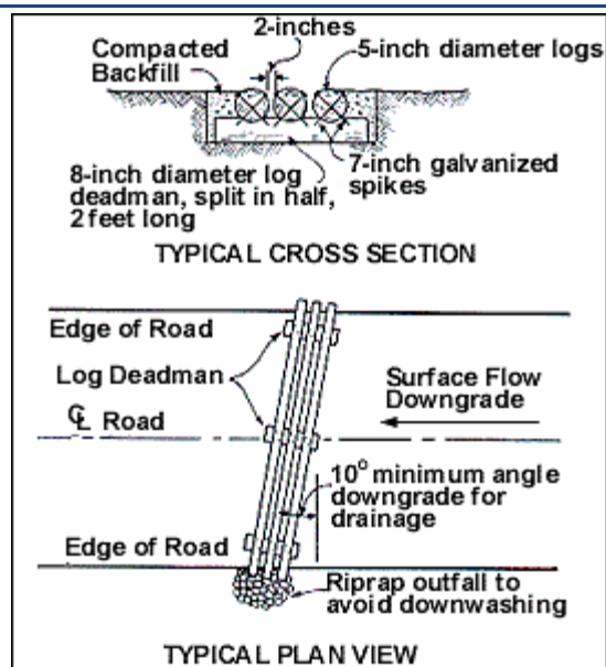
Figure 14. Pole culverts have installation and maintenance requirements similar to those of open-top culverts. (Redrawn and adapted from Michigan Department of Natural Resources 1997, p. 34)
