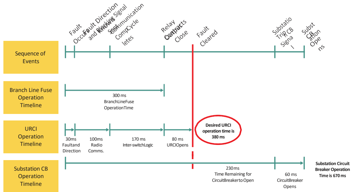
Figure 3.15 Times Associated with Clearing a Fault (URCI = Universal Remote Circuit Interrupter) 39
